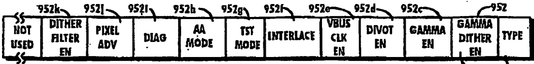
Fig. 35A VIDEO INTERFACE CONTROL REGISTER (R/W)
